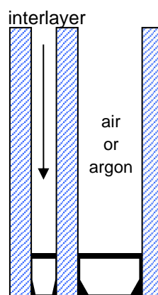
double glazing-construction for outdoor use
